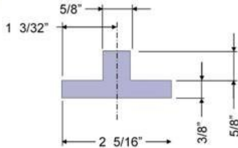
T-Section Gasket installed in a new 72" rubber-lined Durco pressure leaf filter unit:
