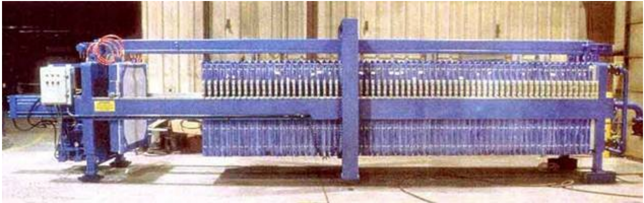
Durco EP Filter Press using hydraulically operated chain-drive filter plate shifter with double pawls
